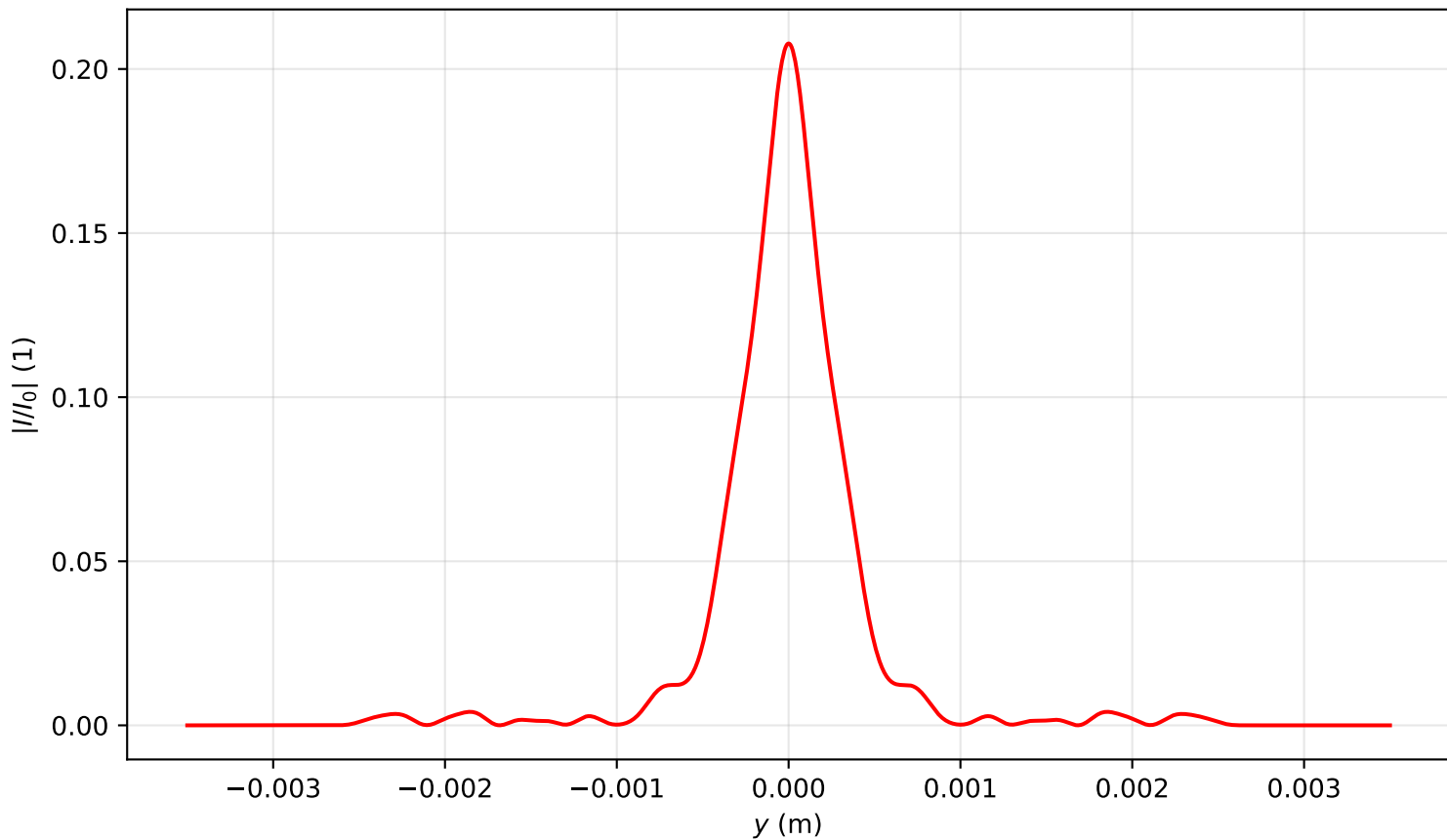
Intensity profile I(x=0, y, z=2.866)/I_0 , P_{in}=6.0P_{cr} , artificial time
